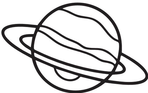
SATURN
